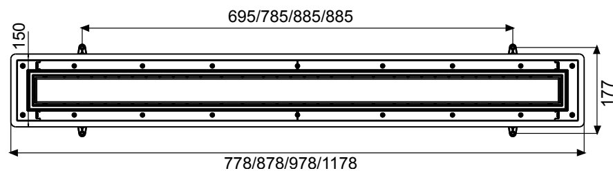
Technical drawing
