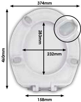
DIAGRAM - SCI11WY Full dimensional details per hinge p33
