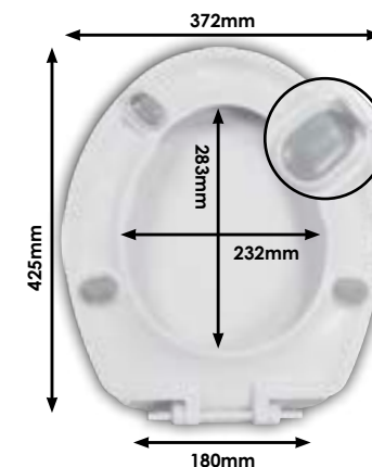
DIAGRAM - SCK11WY Full dimensional details per hinge p33
