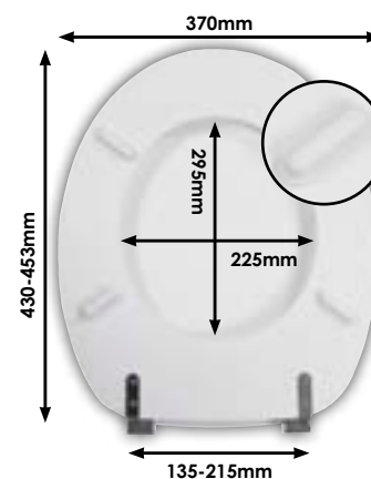
DIAGRAM - 21230004 Full dimensionals details per hinge p33
