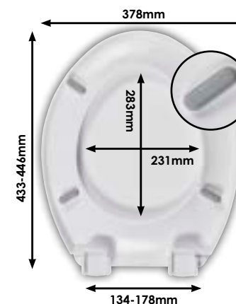
DIAGRAM - SSP11WH Full dimensional details per hinge p31
