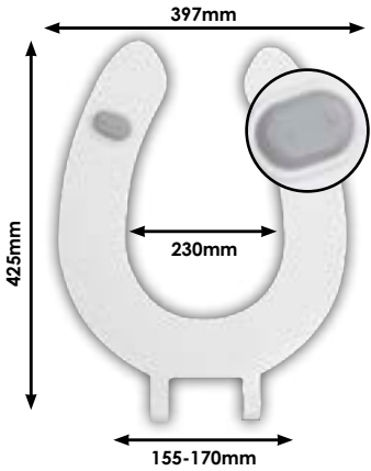
DIAGRAM - SCR53WH Full dimensionals details per hinge p33
