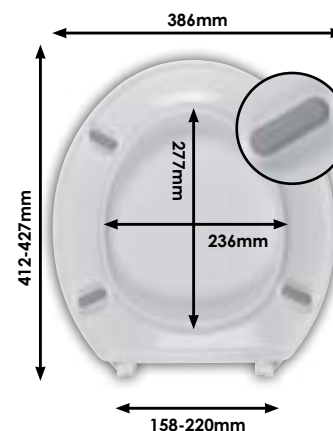
DIAGRAM - 20120361 Full dimensional details per hinge p31
