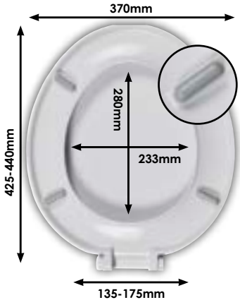
DIAGRAM - SCA11WH Full dimensionalsal details per hinge p31
