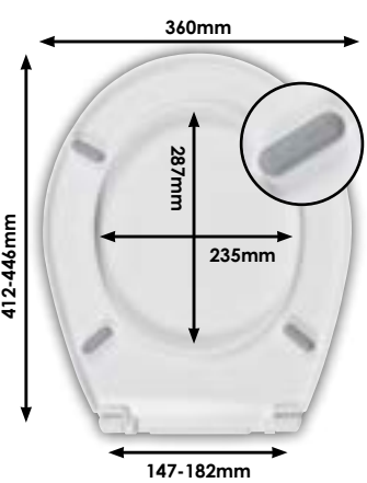
DIAGRAM - SNL11WH Full dimensionals details per hinge p31
