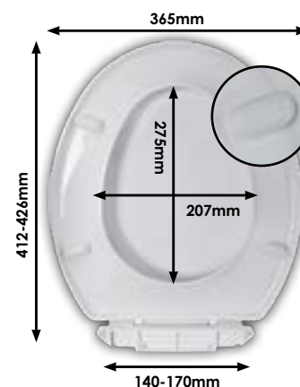
DIAGRAM - 20718747 Full dimensional details per hinge p31
