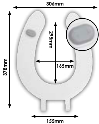
DIAGRAM - SCJ53WH Full dimensionals details per hinge p33
