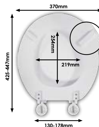
DIAGRAM - 21230001 Full dimensionals details per hinge p33
