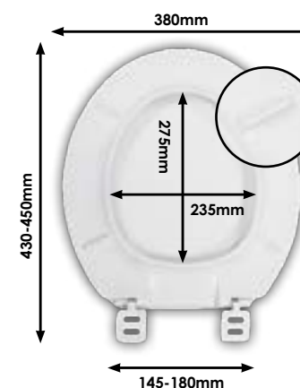
DIAGRAM - SEM11WH Full dimensional details per hinge p31
