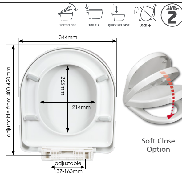
DIAGRAM - 29998023 Full dimensional details per hinge p6
