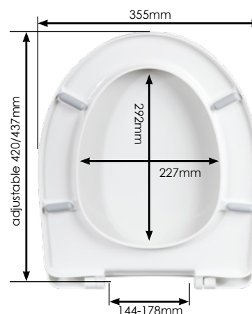
DIAGRAM - 20900008 Full dimensional details per hinge p6
